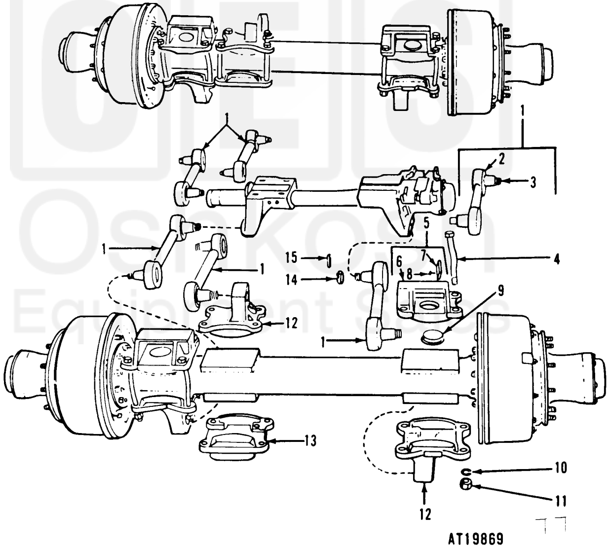
Figure 37. Torque rods, spring guide brackets, and attaching parts—exploded view.
